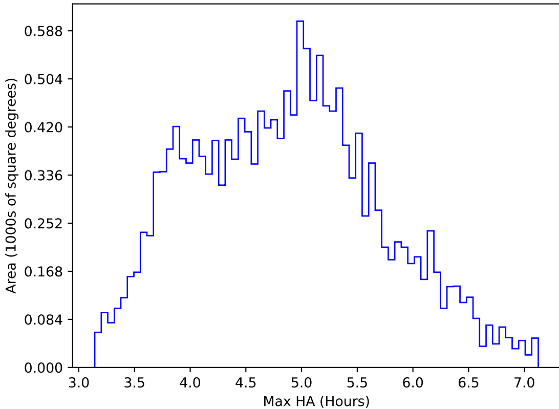
too_elab_r32_d3_gz_v3.4_10yrs WFD i band: Max HA
