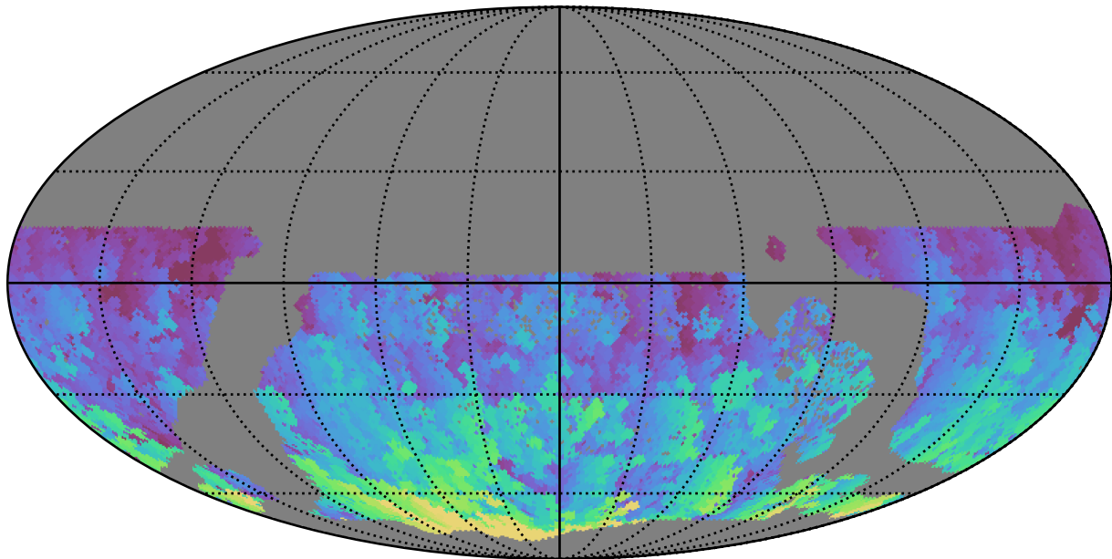
too_elab_r32_d3_gz_v3.4_10yrs WFD g band: Max HA
