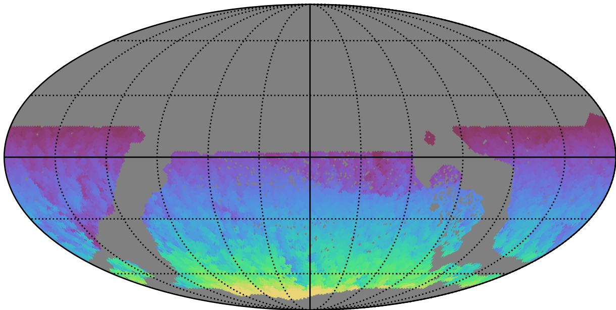
too_elab_r32_d3_gz_v3.4_10yrs WFD all bands: Max HA
