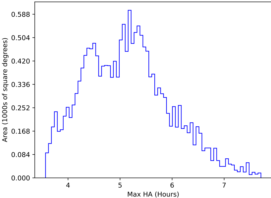
too_elab_r32_d3_gz_v3.4_10yrs WFD all bands: Max HA
