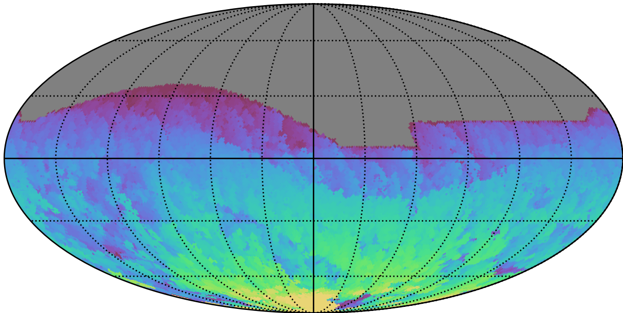
too_elab_r32_d3_gz_v3.4_10yrs All sky z band: Max HA
