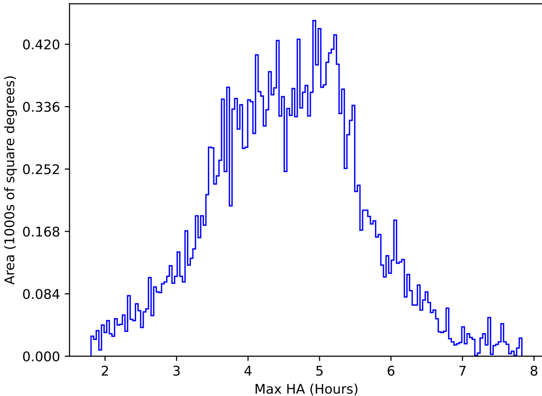
too_elab_r32_d3_gz_v3.4_10yrs All sky z band: Max HA
