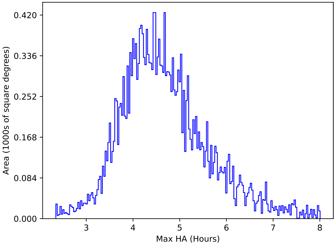
too_elab_r32_d3_gz_v3.4_10yrs All sky y band: Max HA
