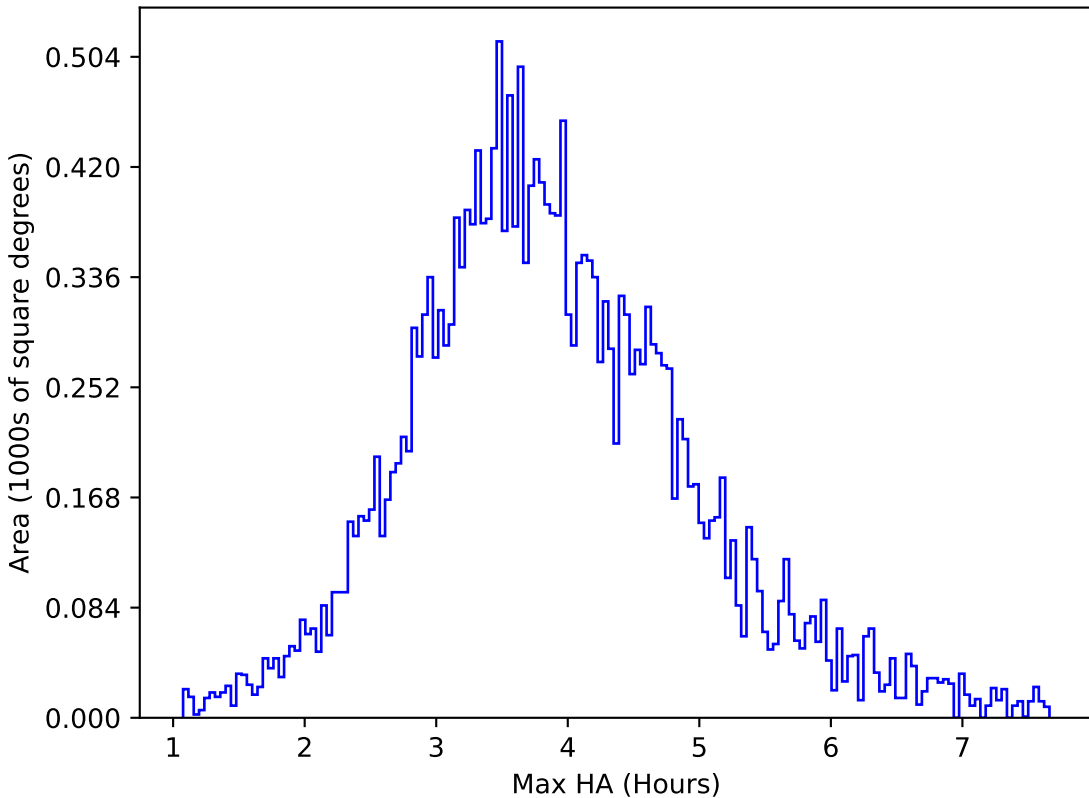
too_elab_r32_d3_gz_v3.4_10yrs All sky u band: Max HA
