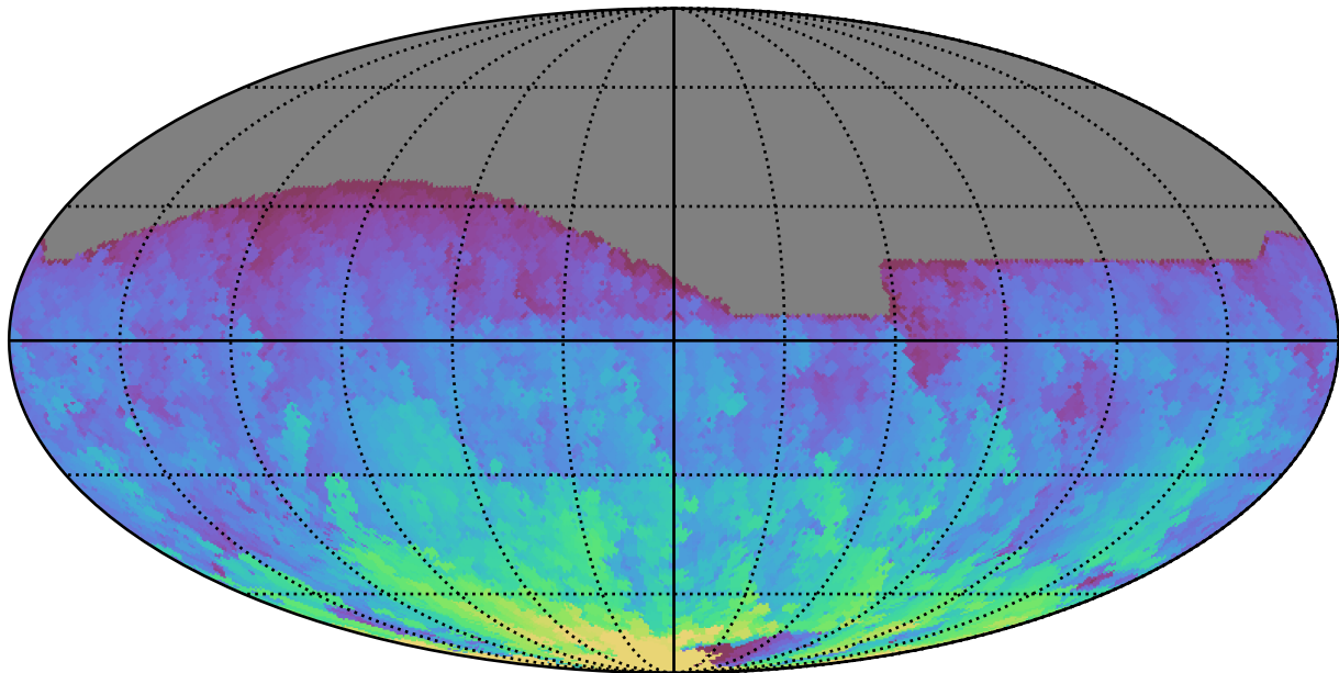
too_elab_r32_d3_gz_v3.4_10yrs All sky r band: Max HA
