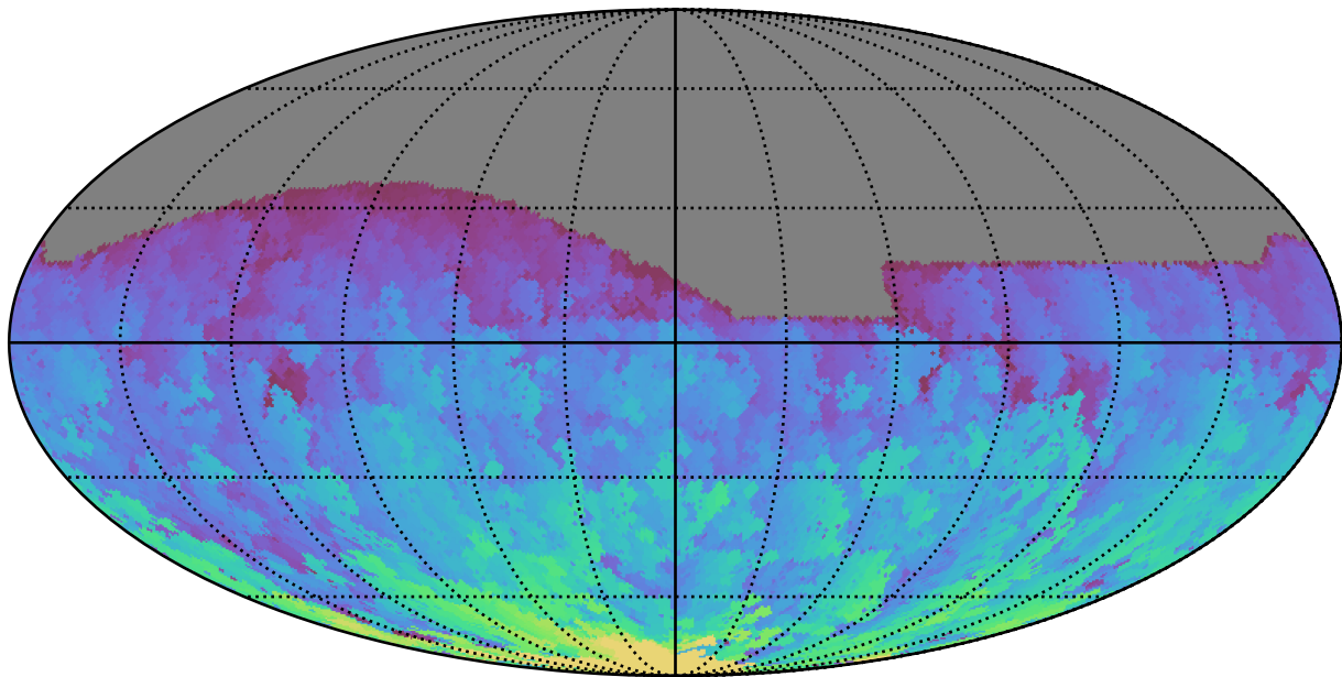
too_elab_r32_d3_gz_v3.4_10yrs All sky g band: Max HA
