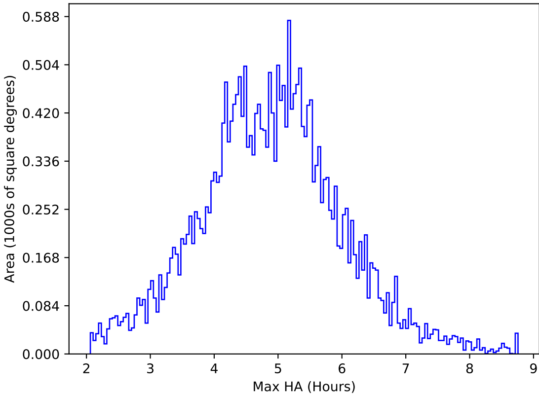
too_elab_r32_d3_gz_v3.4_10yrs All sky all bands: Max HA
