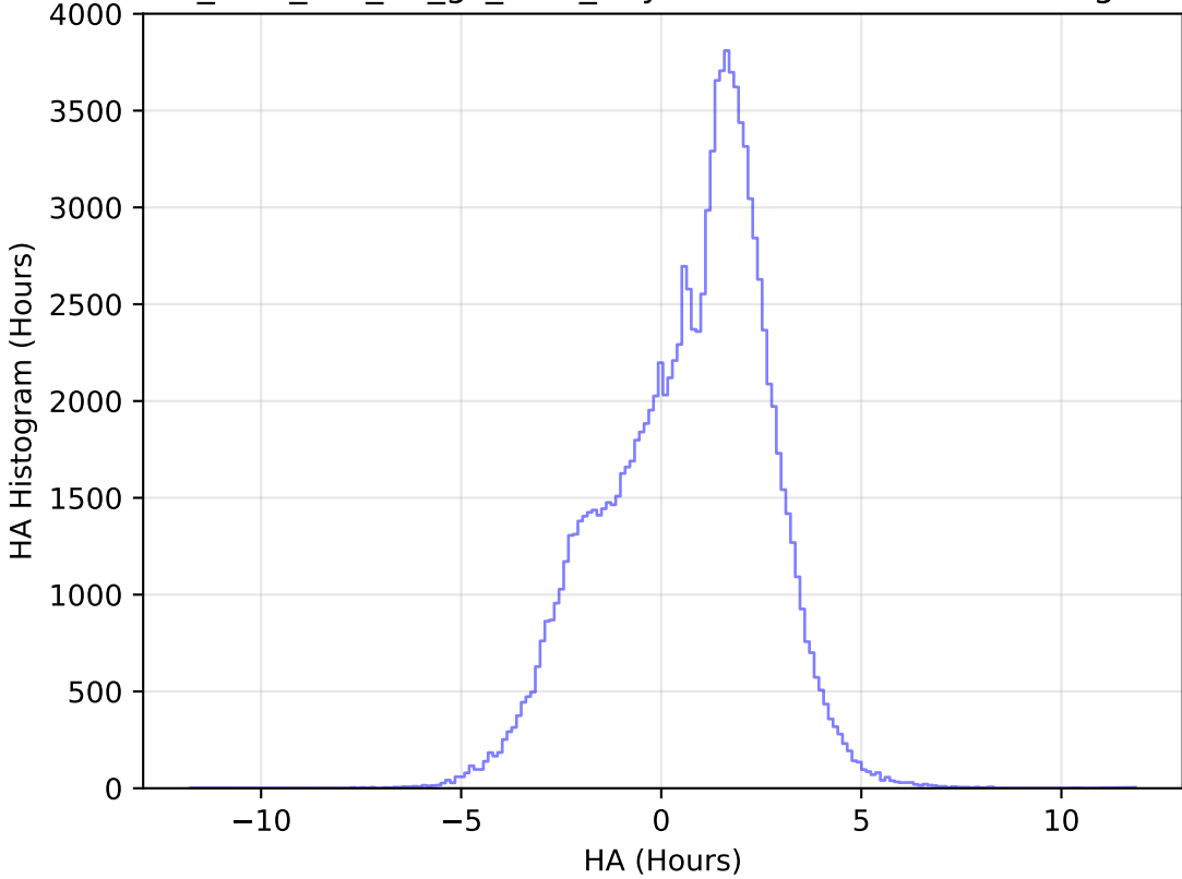
too_elab_r32_d3_gz_v3.4_10yrs WFD u band: HA Histogram
