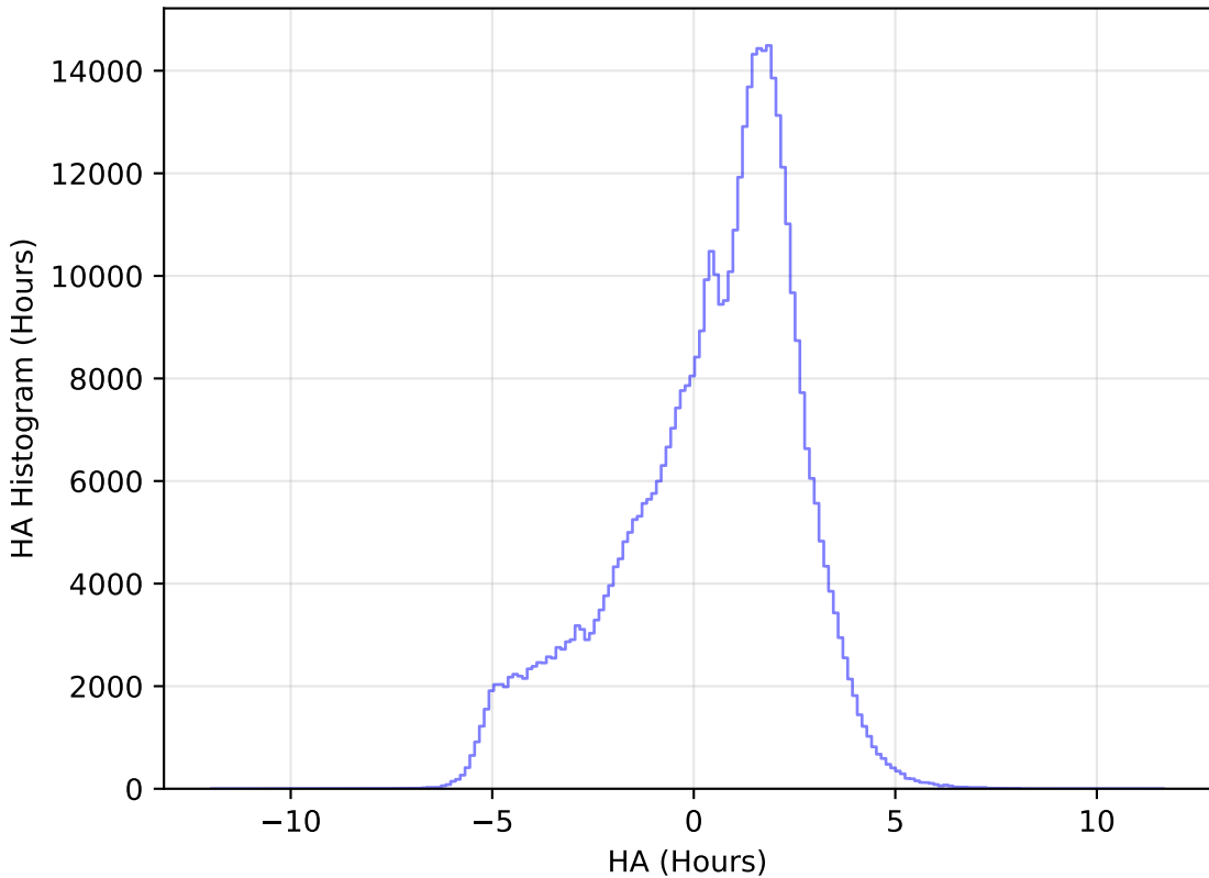
too_elab_r32_d3_gz_v3.4_10yrs WFD r band: HA Histogram
