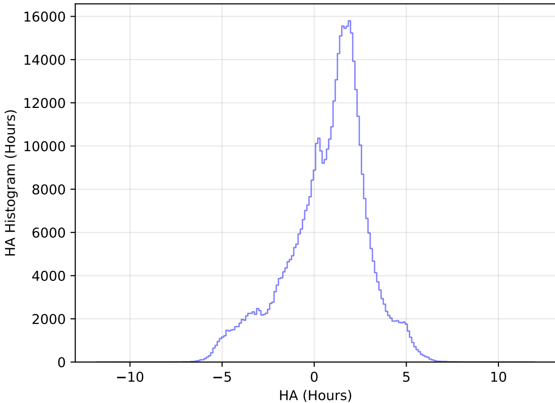
too_elab_r32_d3_gz_v3.4_10yrs WFD i band: HA Histogram
