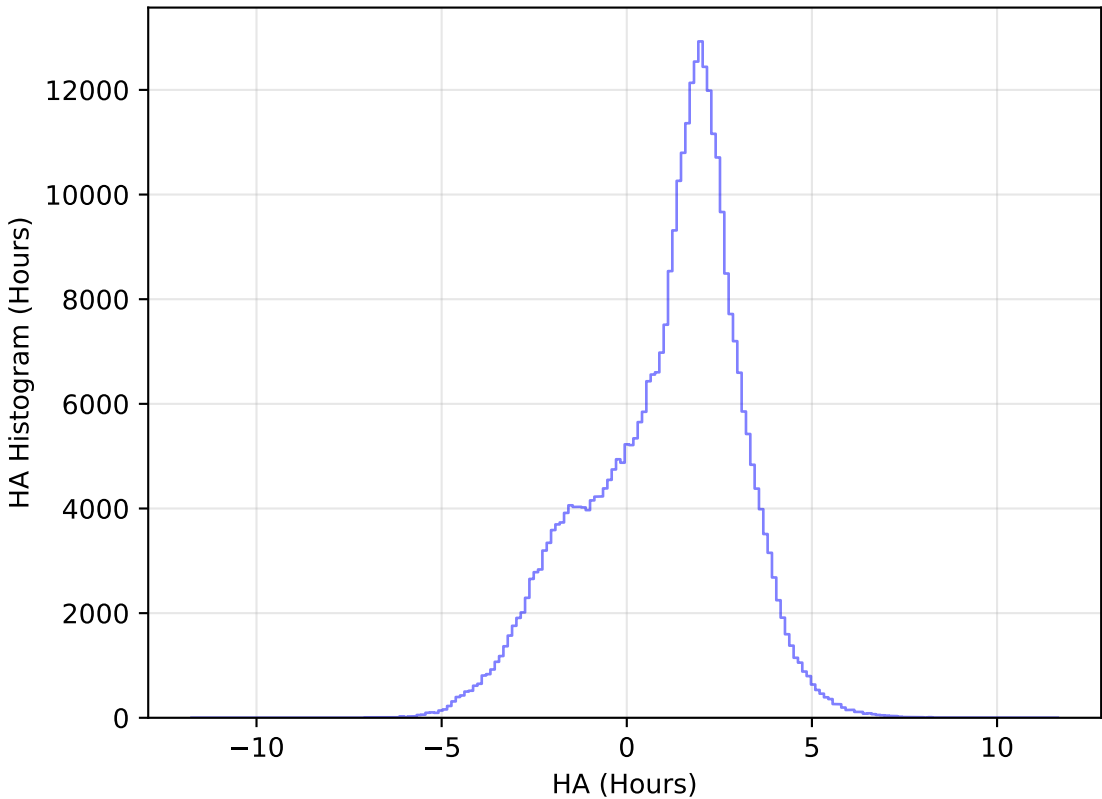
too_elab_r32_d3_gz_v3.4_10yrs All sky y band: HA Histogram
