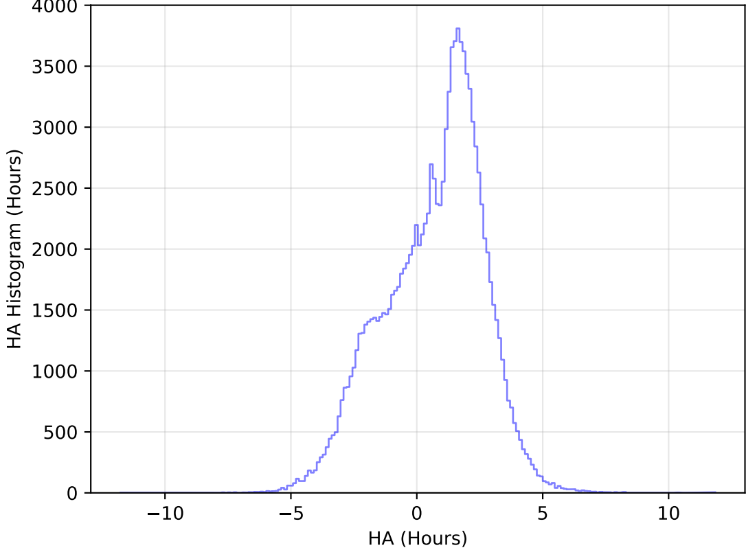
too_elab_r32_d3_gz_v3.4_10yrs All sky u band: HA Histogram
