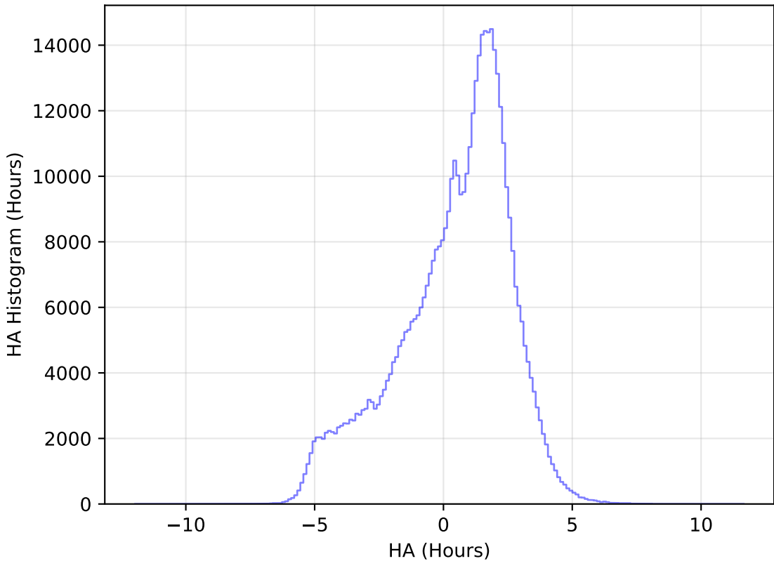
too_elab_r32_d3_gz_v3.4_10yrs All sky r band: HA Histogram
