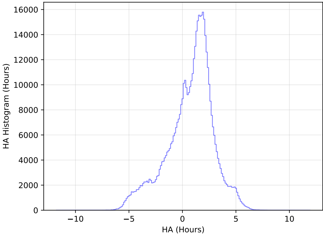
too_elab_r32_d3_gz_v3.4_10yrs All sky i band: HA Histogram
