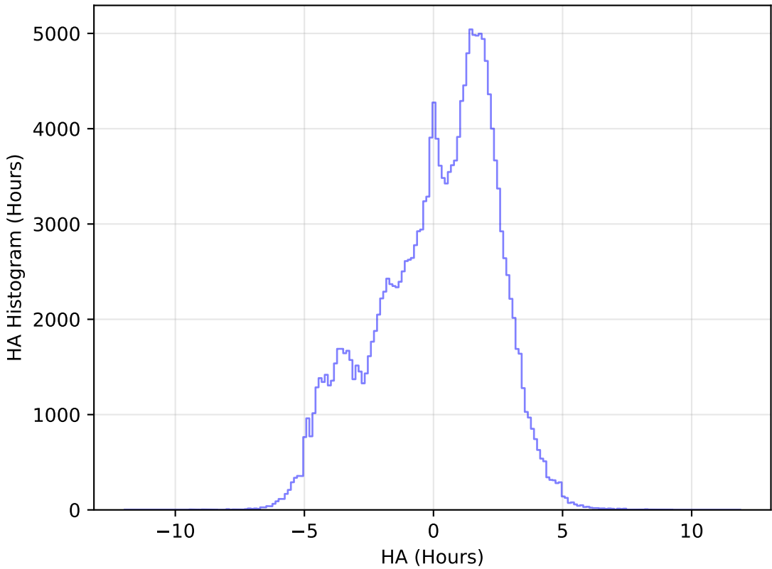
too_elab_r32_d3_gz_v3.4_10yrs All sky g band: HA Histogram
