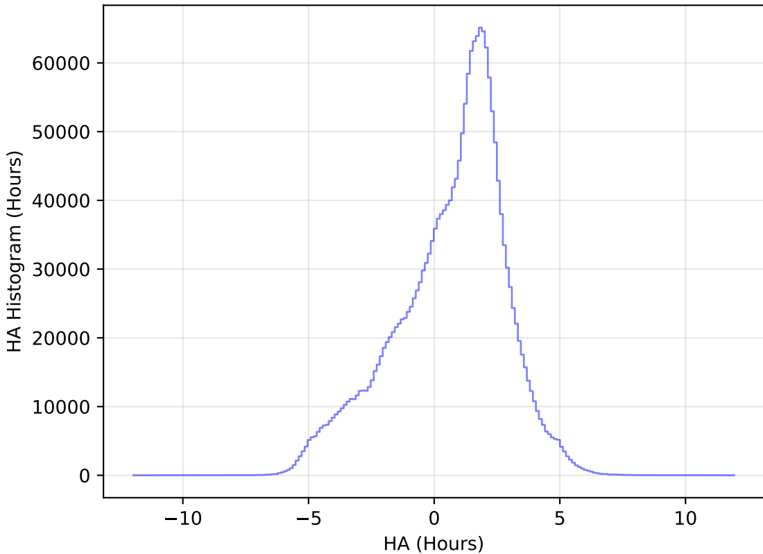
too_elab_r32_d3_gz_v3.4_10yrs All sky all bands: HA Histogram
