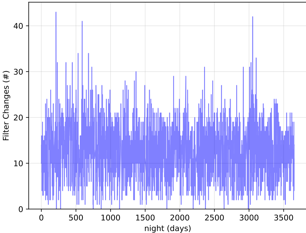
too_elab_r32_d3_gz_v3.4_10yrs Per Night: Filter Changes
