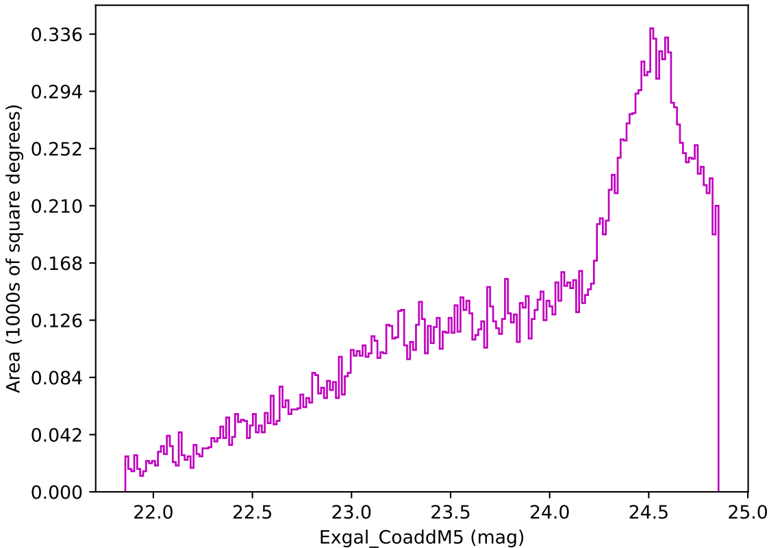
too_elab_r32_d3_gz_v3.4_10yrs Yr 3-4 z band: Exgal_CoaddM5
