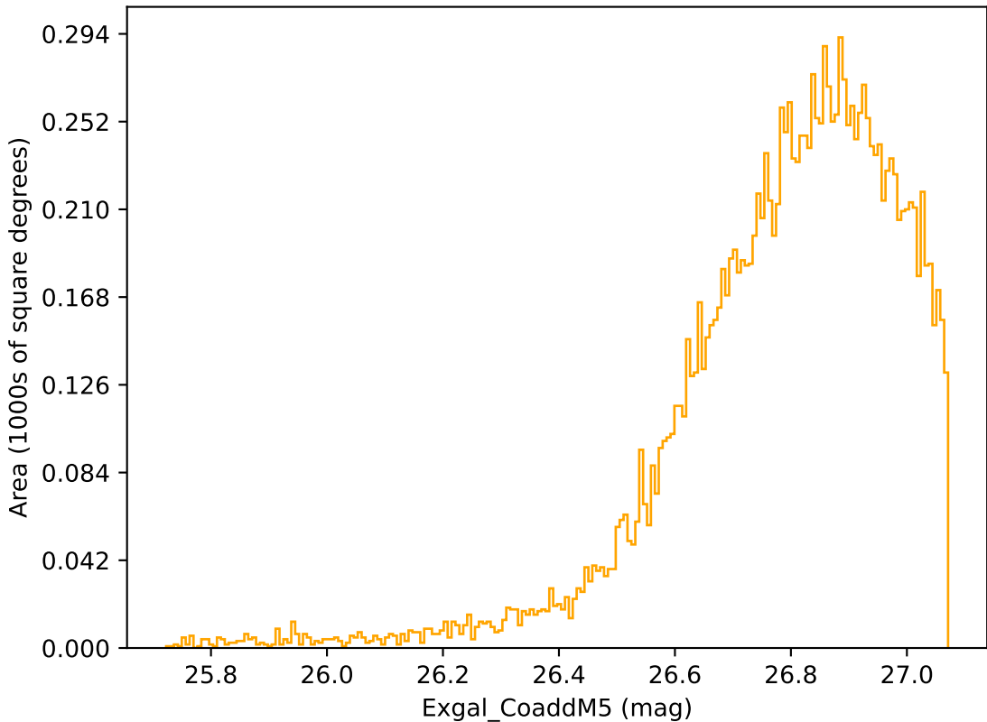
too_elab_r32_d3_gz_v3.4_10yrs WFD r band: Exgal_CoaddM5
