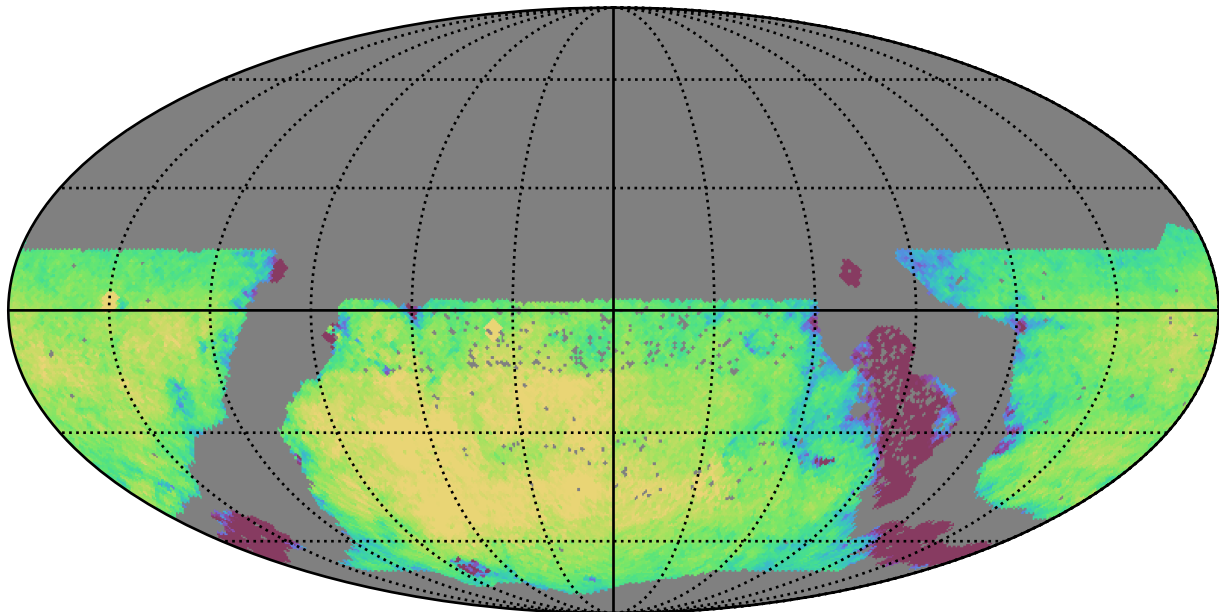
too_elab_r32_d3_gz_v3.4_10yrs WFD g band: Exgal_CoaddM5
