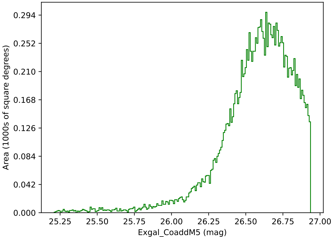
too_elab_r32_d3_gz_v3.4_10yrs WFD g band: Exgal_CoaddM5
