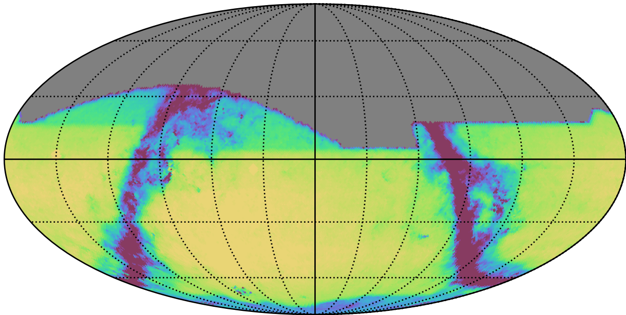
too_elab_r32_d3_gz_v3.4_10yrs All sky r band: Exgal_CoaddM5
