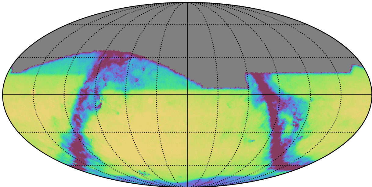
too_elab_r32_d3_gz_v3.4_10yrs All sky i band: Exgal_CoaddM5
