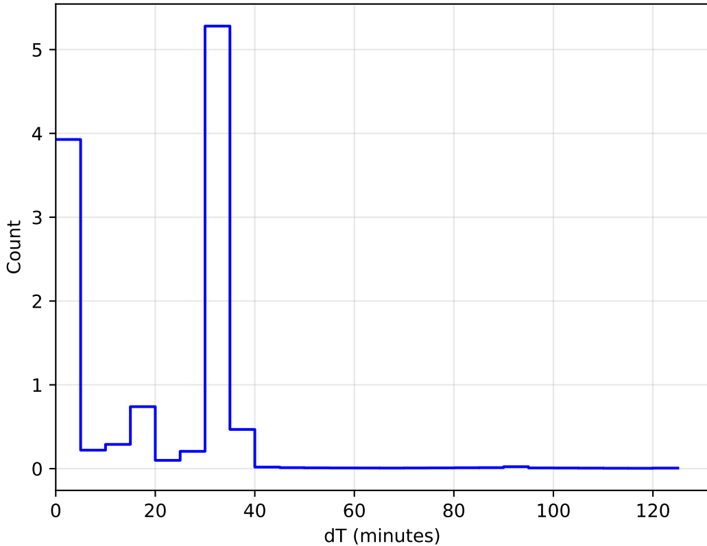
too_elab_r32_d3_gz_v3.4_10yrs WFD: DeltaT Histogram
