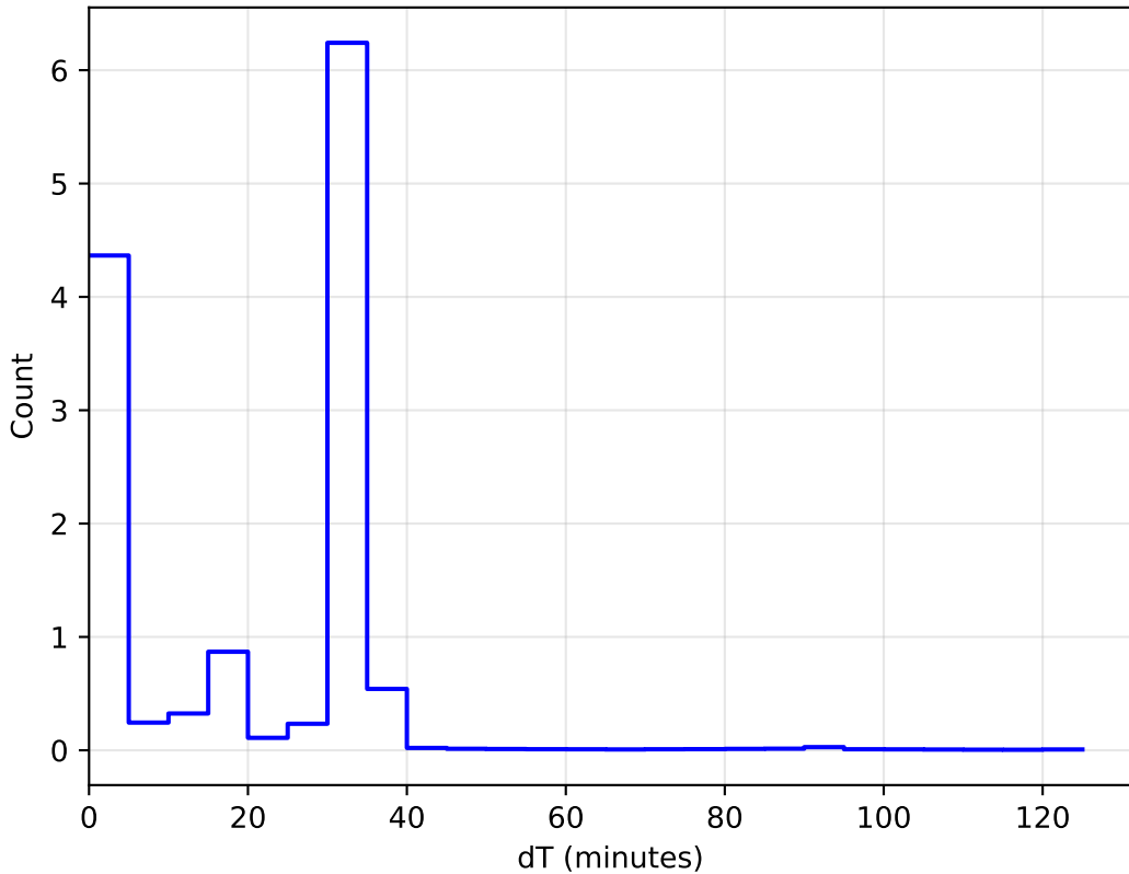
too_elab_r32_d3_gz_v3.4_10yrs All sky: DeltaT Histogram 1e6
