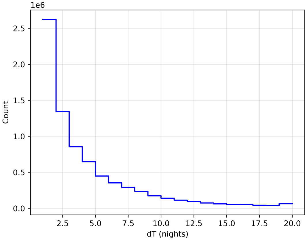
too_elab_r32_d3_gz_v3.4_10yrs WFD all bands: DeltaNight Histogram
