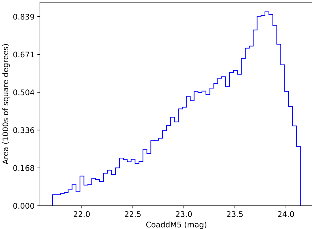
too_elab_r32_d3_gz_v3.4_10yrs Yr 3-4 y band: CoaddM5
