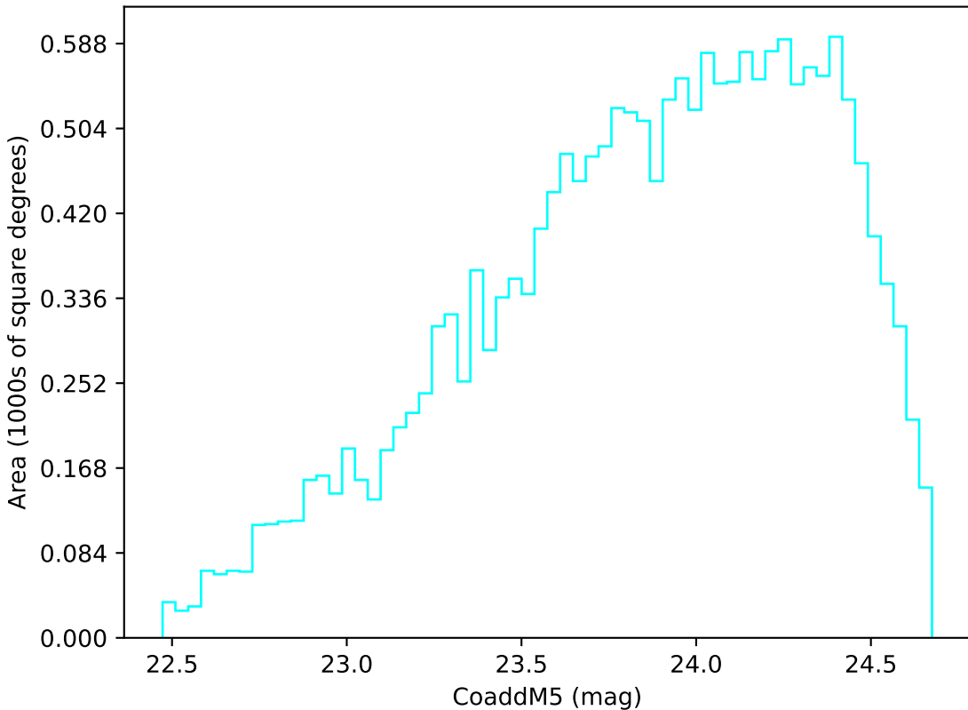
too_elab_r32_d3_gz_v3.4_10yrs Yr 3-4 u band: CoaddM5
