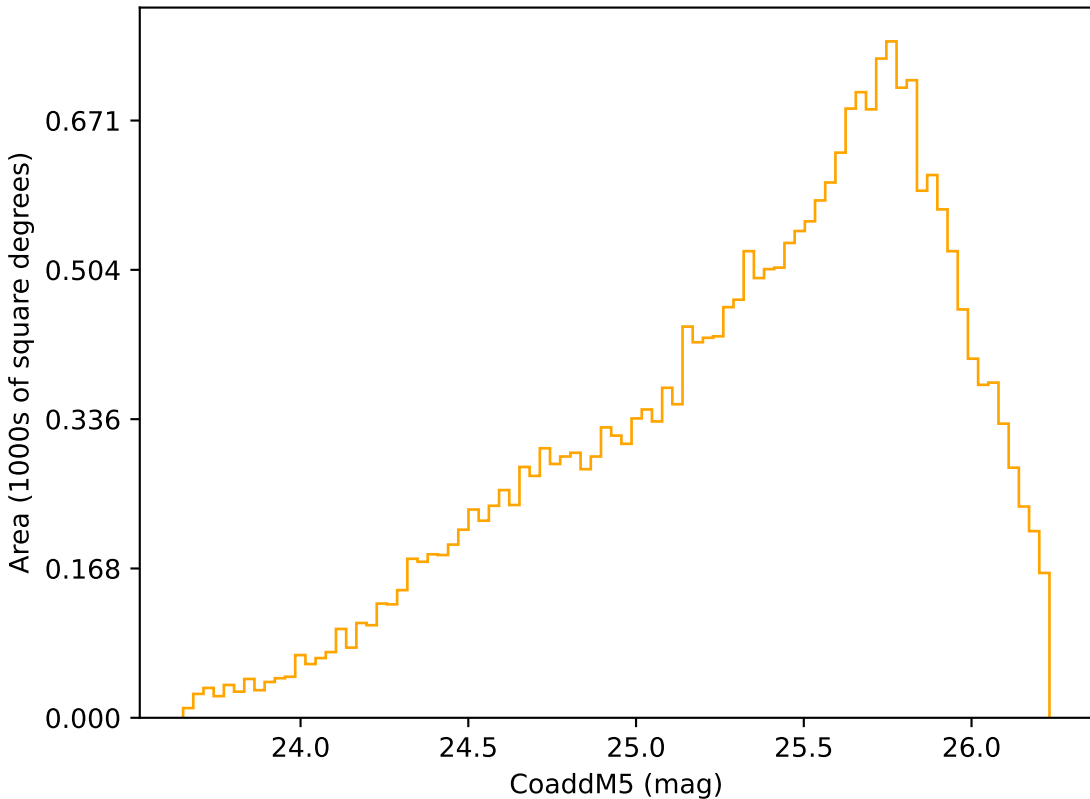
too_elab_r32_d3_gz_v3.4_10yrs Yr 3-4 r band: CoaddM5
