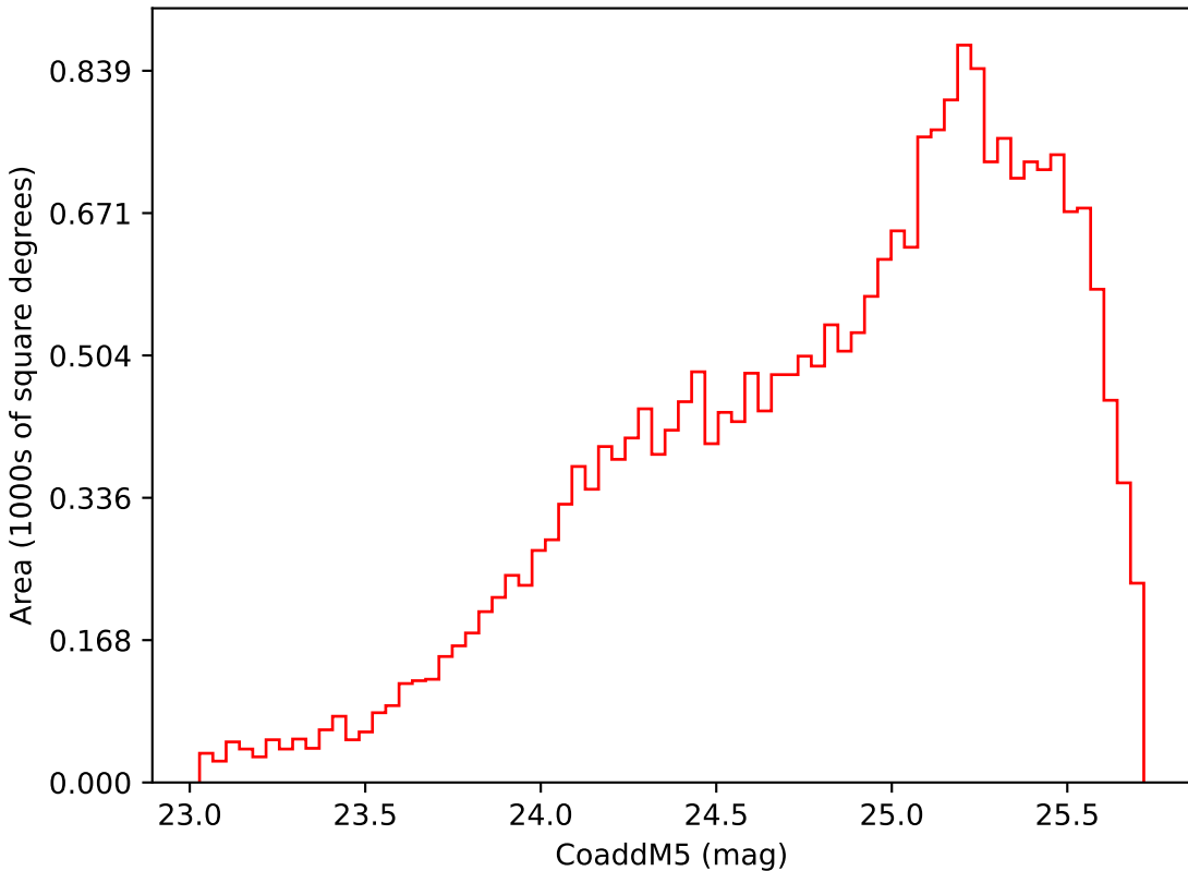
too_elab_r32_d3_gz_v3.4_10yrs Yr 3-4 i band: CoaddM5
