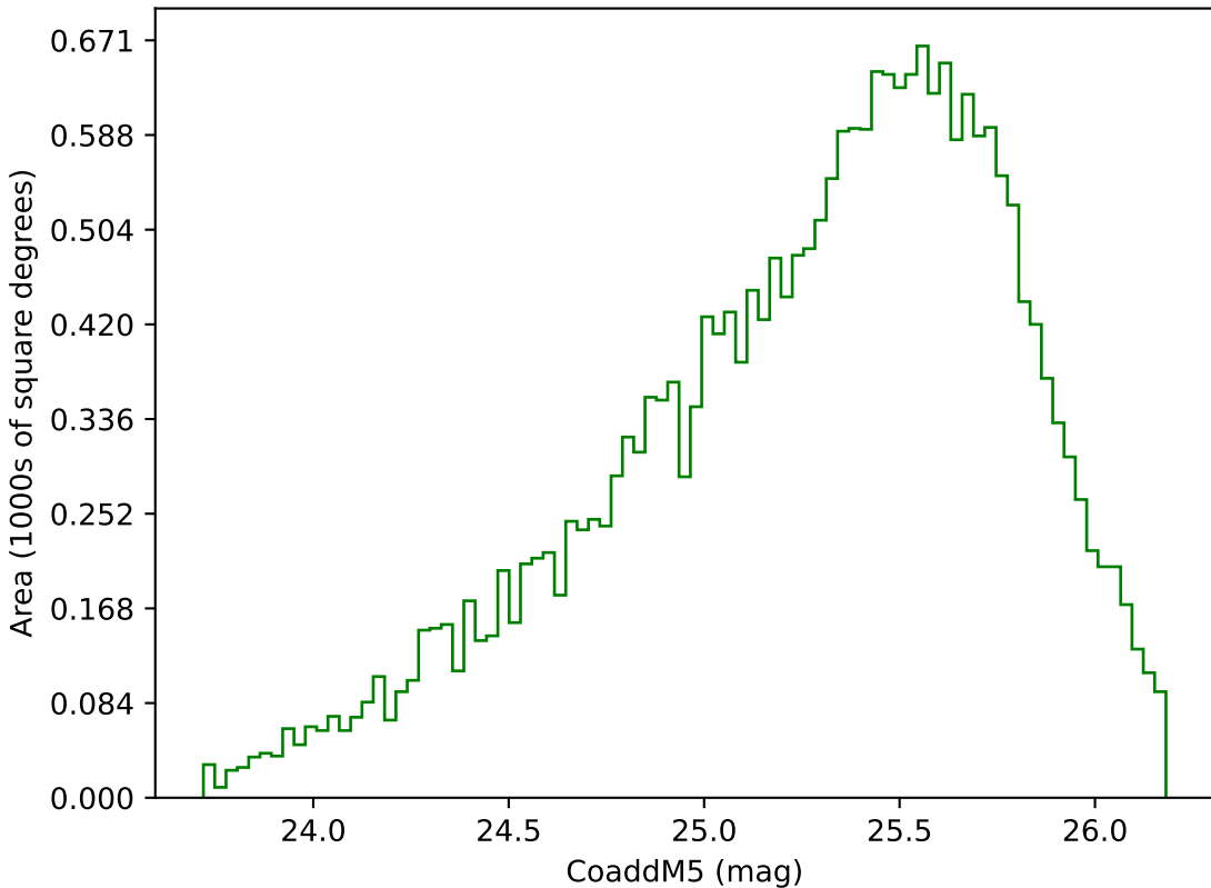
too_elab_r32_d3_gz_v3.4_10yrs Yr 3-4 g band: CoaddM5
