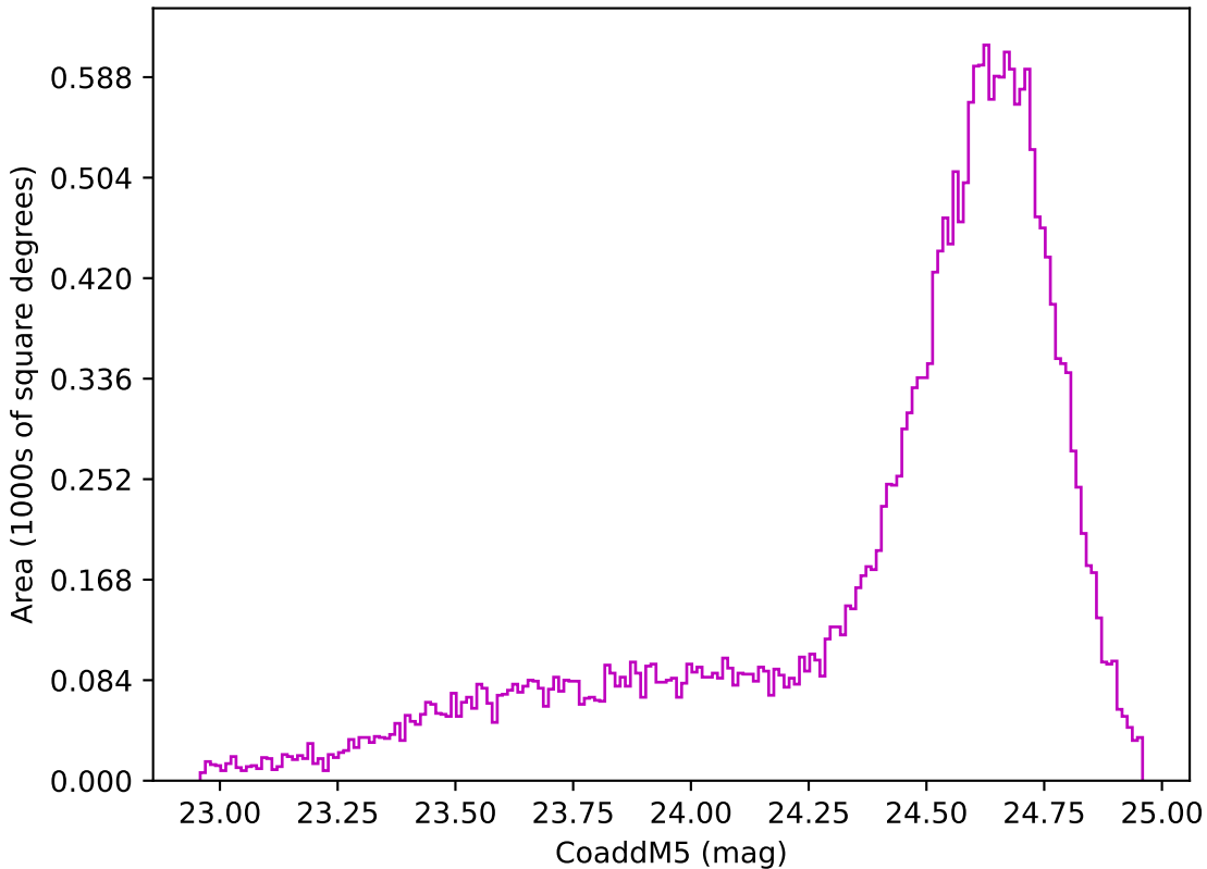
too_elab_r32_d3_gz_v3.4_10yrs Yr 1 z band: CoaddM5
