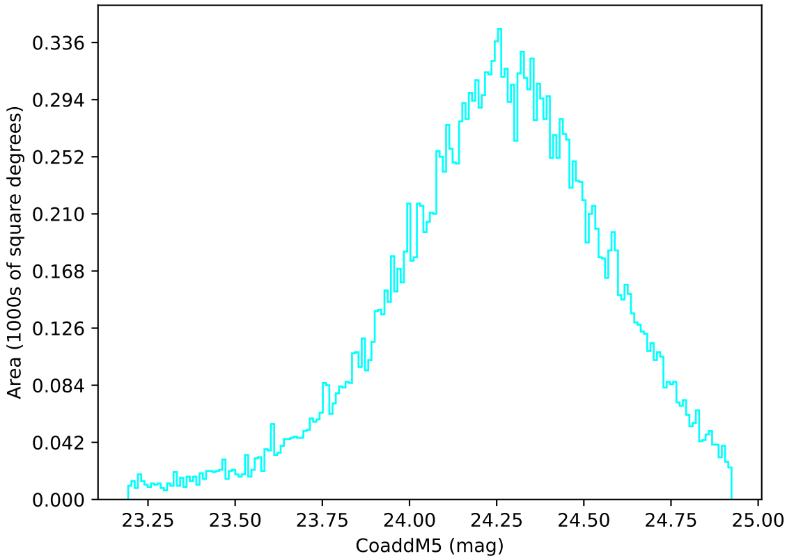
too_elab_r32_d3_gz_v3.4_10yrs Yr 1 u band: CoaddM5
