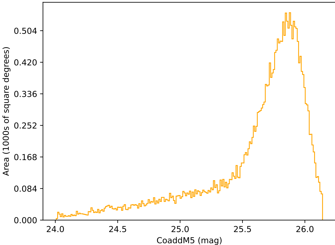
too_elab_r32_d3_gz_v3.4_10yrs Yr 1 r band: CoaddM5
