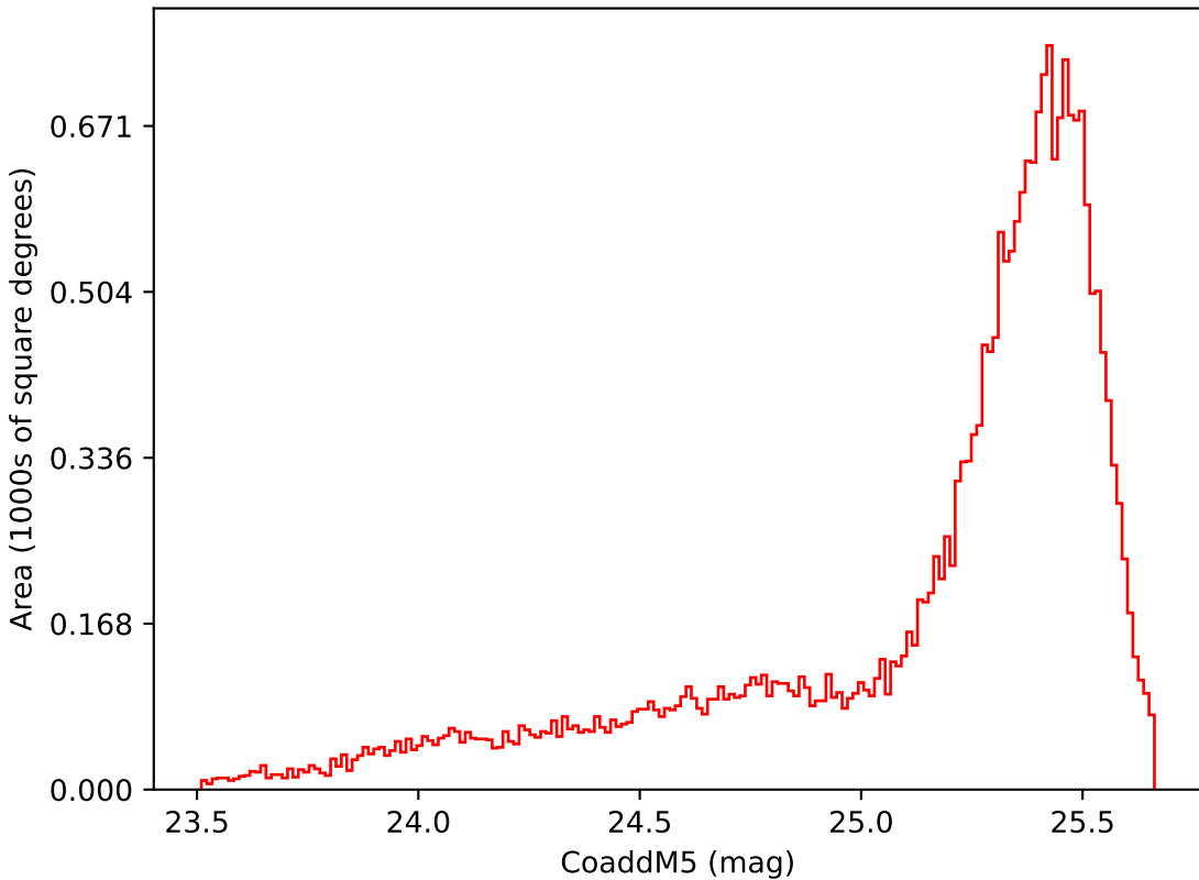
too_elab_r32_d3_gz_v3.4_10yrs Yr 1 i band: CoaddM5
