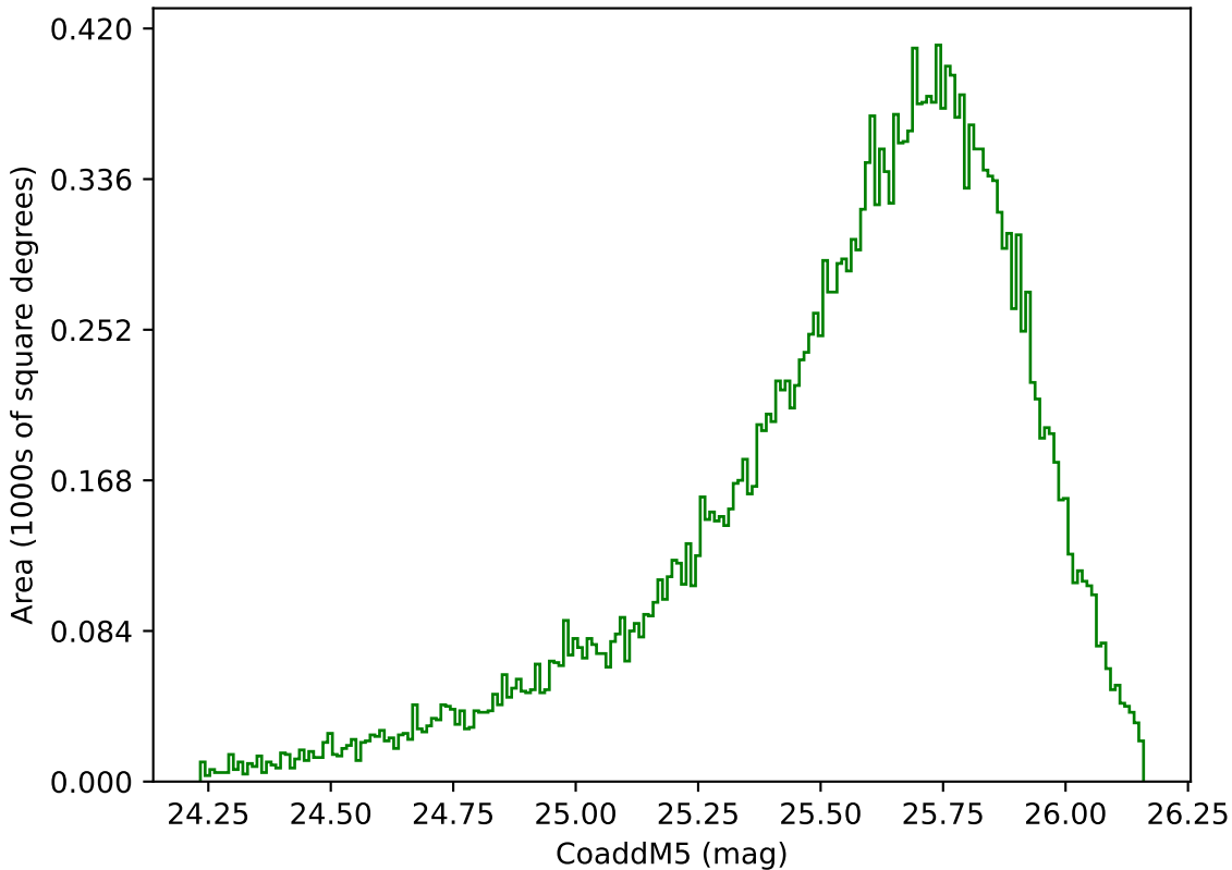
too_elab_r32_d3_gz_v3.4_10yrs Yr 1 g band: CoaddM5
