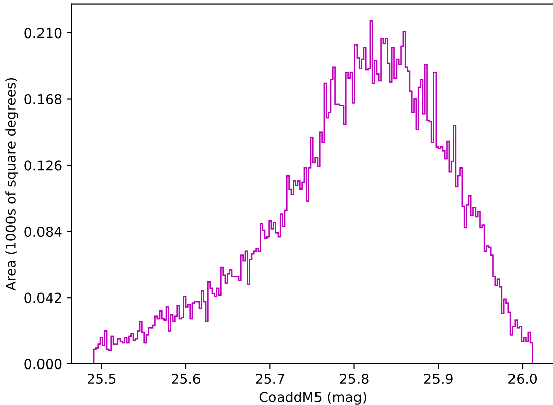
too_elab_r32_d3_gz_v3.4_10yrs WFD z band: CoaddM5
