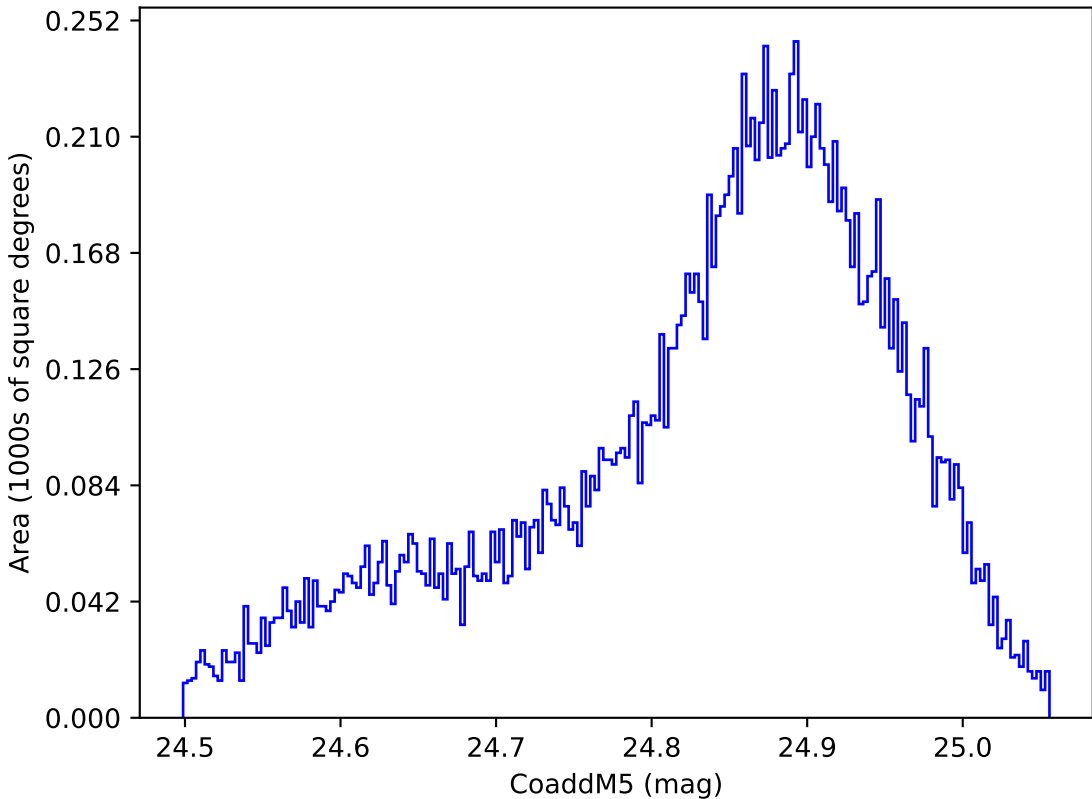
too_elab_r32_d3_gz_v3.4_10yrs WFD y band: CoaddM5
