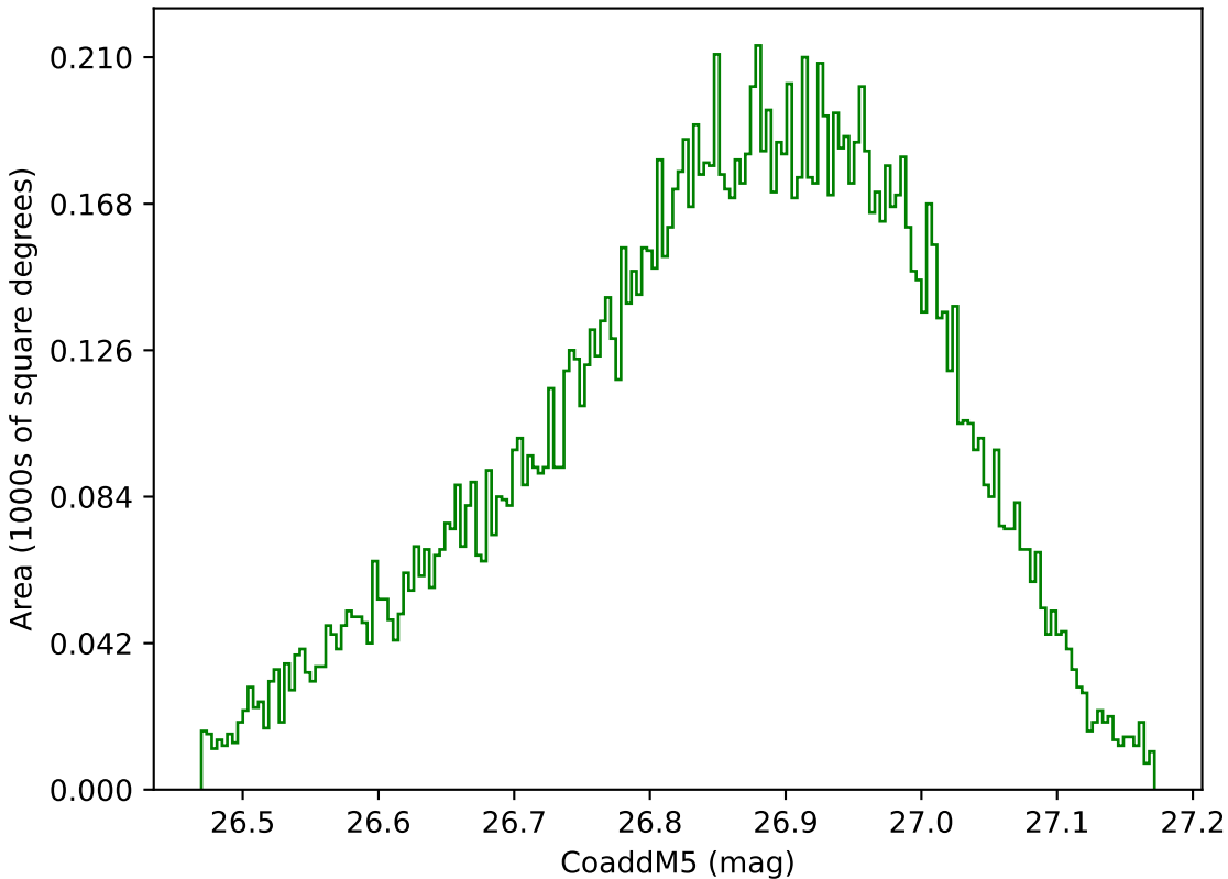
too_elab_r32_d3_gz_v3.4_10yrs WFD g band: CoaddM5
