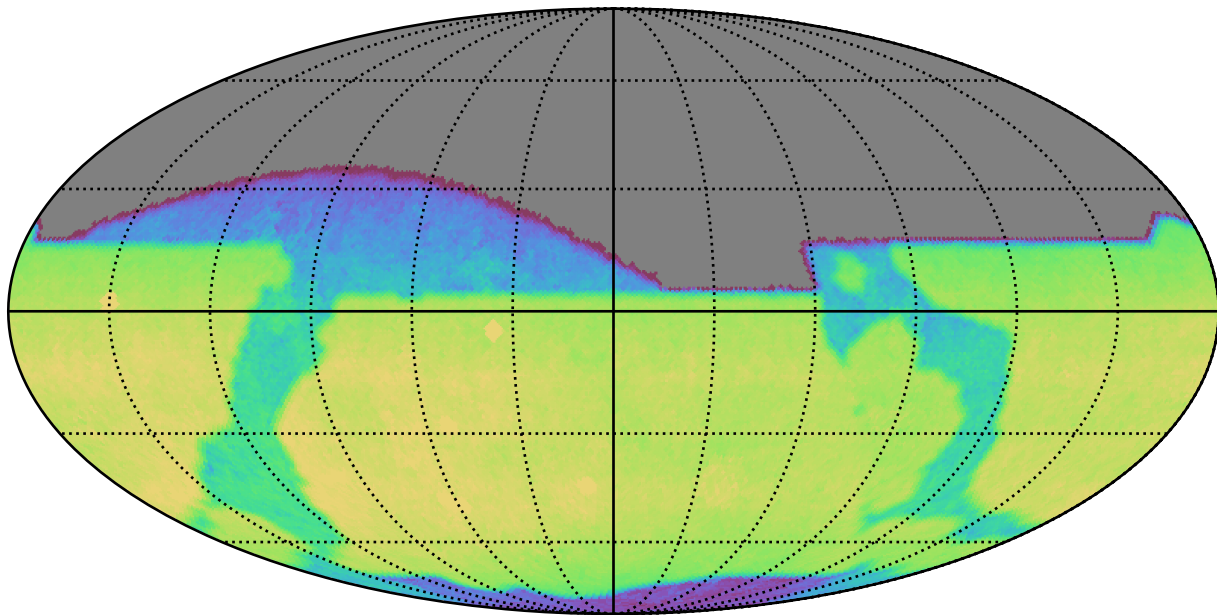
too_elab_r32_d3_gz_v3.4_10yrs All sky z band: CoaddM5
