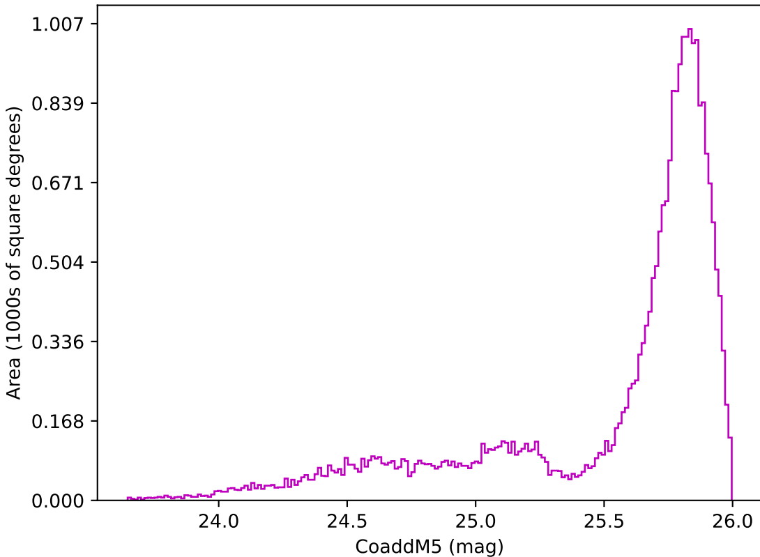
too_elab_r32_d3_gz_v3.4_10yrs All sky z band: CoaddM5
