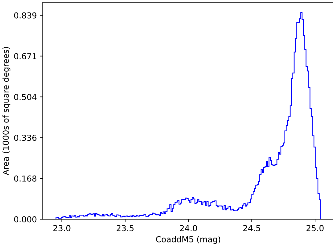
too_elab_r32_d3_gz_v3.4_10yrs All sky y band: CoaddM5
