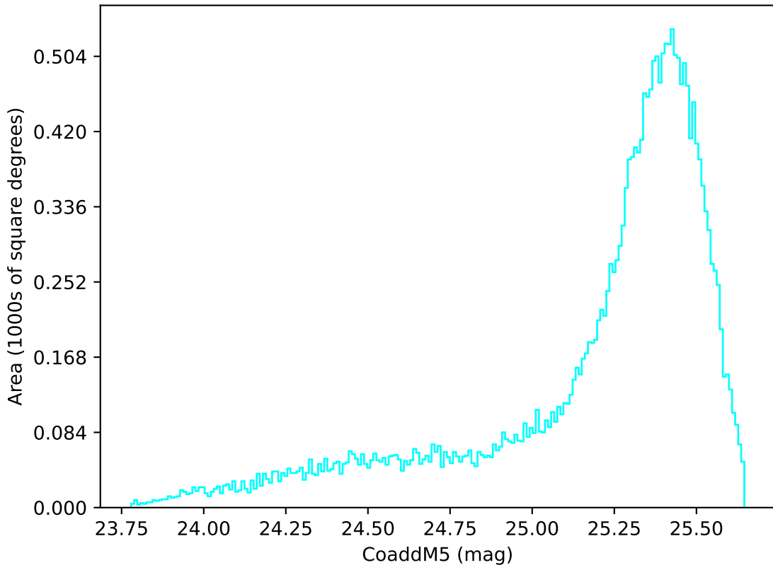
too_elab_r32_d3_gz_v3.4_10yrs All sky u band: CoaddM5
