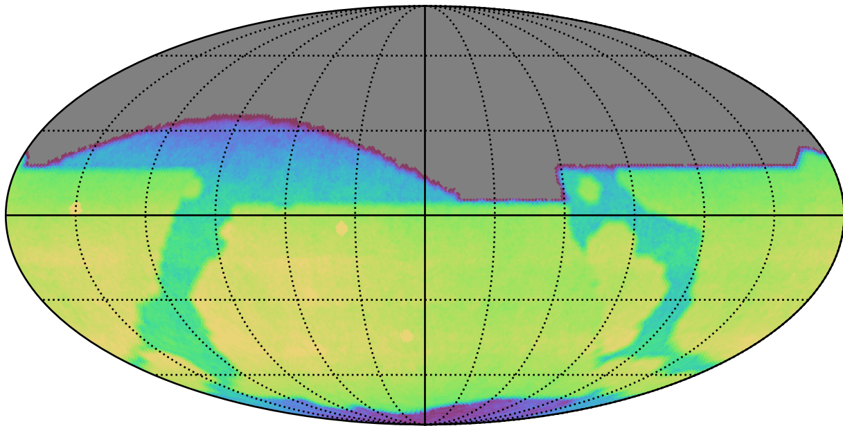
too_elab_r32_d3_gz_v3.4_10yrs All sky r band: CoaddM5
