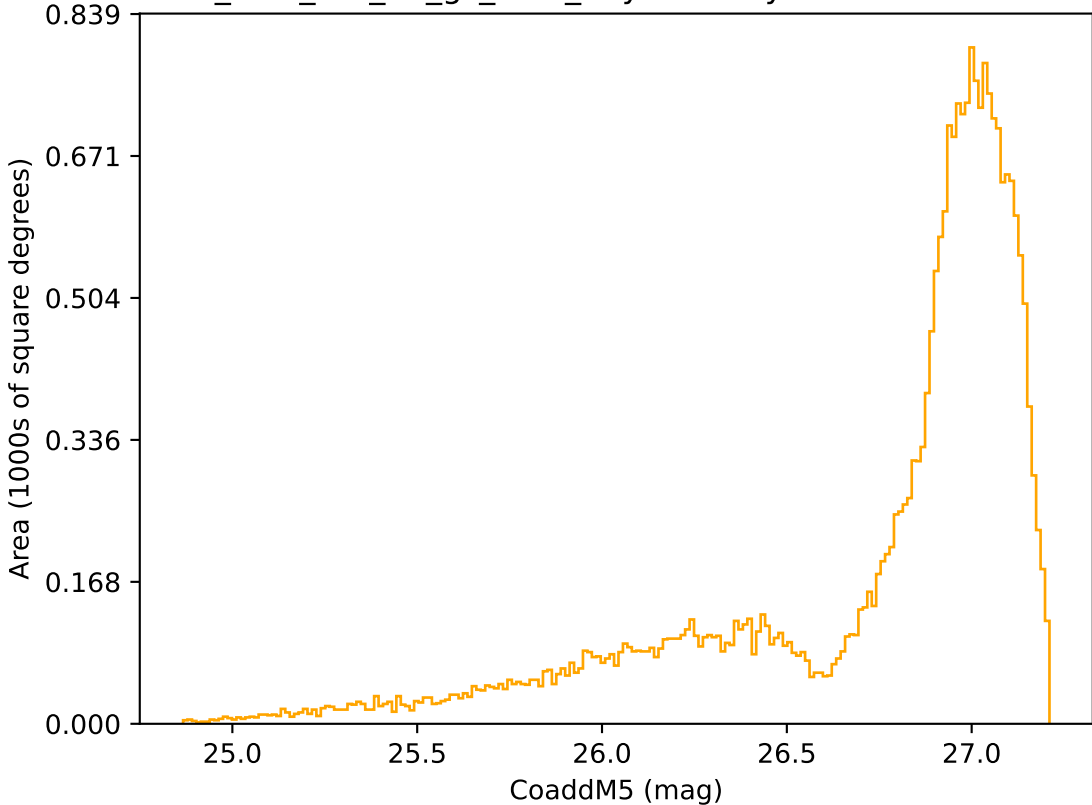
too_elab_r32_d3_gz_v3.4_10yrs All sky r band: CoaddM5
