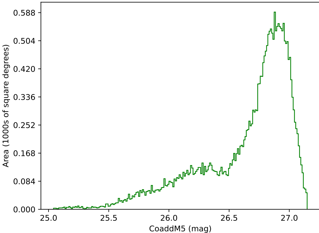
too_elab_r32_d3_gz_v3.4_10yrs All sky g band: CoaddM5
